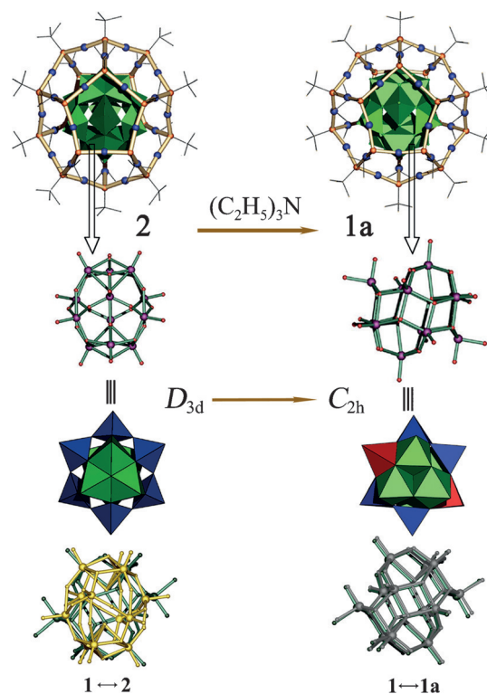
Figure 2. First row compares the [\text{Ag}_{30}(\text{tBuS})_{20}]^{10+} shells (ball-and-stick models) wrapping tightly around their [\text{V}_{10}^{\text{V}}\text{V}_{2}^{\text{IV}}\text{O}_{34}]^{10-} cores (polyhedral models) of the host-guest cluster assemblies in 2 and 1a viewed down their respective idealized S_{10} symmetry axes. The second and third rows compare the two polyoxovanadate cores viewed laterally (ball-and-stick) and in projection (polyhedral). In the last row, the left-hand side shows an overlap of the [\text{V}_{10}^{\text{V}}\text{V}_{2}^{\text{IV}}\text{O}_{34}]^{10-} core in 1 (dark green) and [\text{V}_{10}^{\text{V}}\text{V}_{2}^{\text{IV}}\text{O}_{34}]^{10-} core 2 (yellow); the right-hand side shows a slightly offset overlap of the [\text{V}_{10}^{\text{V}}\text{V}_{2}^{\text{IV}}\text{O}_{34}]^{10-} core in 1 (dark green) and [\text{V}_{10}^{\text{V}}\text{V}_{2}^{\text{IV}}\text{O}_{34}]^{10-} core 1a (gray). Color code for ball-and-stick models: Ag blue; V purple; S orange; O red; C gray.
